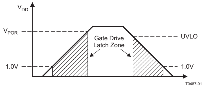
Figure 10. UVLO Operation
